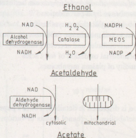
Fig. 2. Pathways of ethanol metabolism
