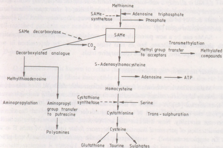
Fig. 13. Metabolic fate of S-adenosyl-L-methionine (SAME)
