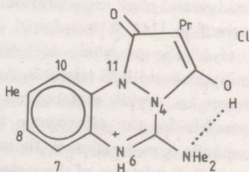
Fig. 1. Structure of the benzotriazine oxide NSAID, azapropazone (HCl salt)
