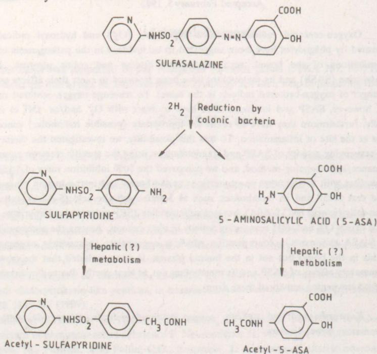
Fig. 1. The fate of orally administered sulfasalazine in the human body
