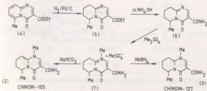
Fig. 2. Syntheses of CHINOIN-105 (2) and CHINOIN-127 (3)
