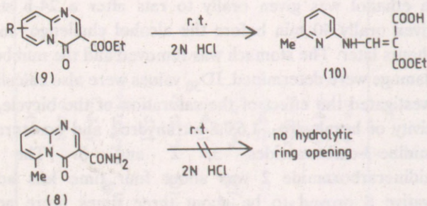
Fig. 5. Hydrolytic ring opening gives highly toxic 2-pyridylaminomethylenemalonic acid derivative
