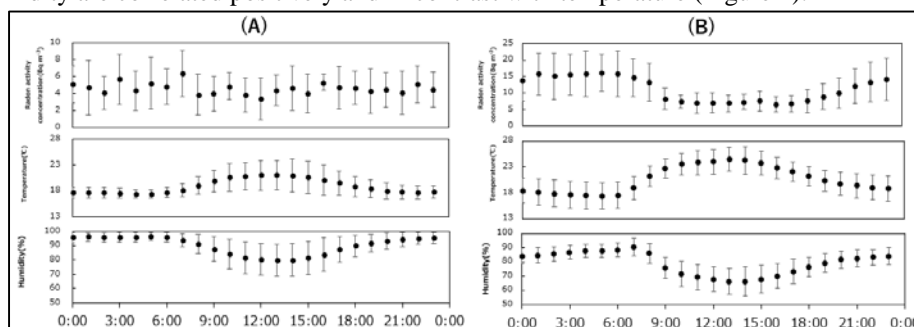
Figure 1: Variation of radon concentration, temperature and humidity measured using AlphaGUARD at (A) Chitoksetai district and (B) Chikagawa district
