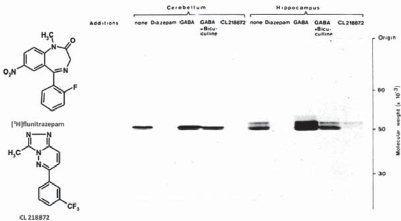
Figure 1: Structural formula of flunitrazepam and Cl 218872, and molecular heterogeneity of benzodiazepine receptors. Figure modified from Ref 8.
