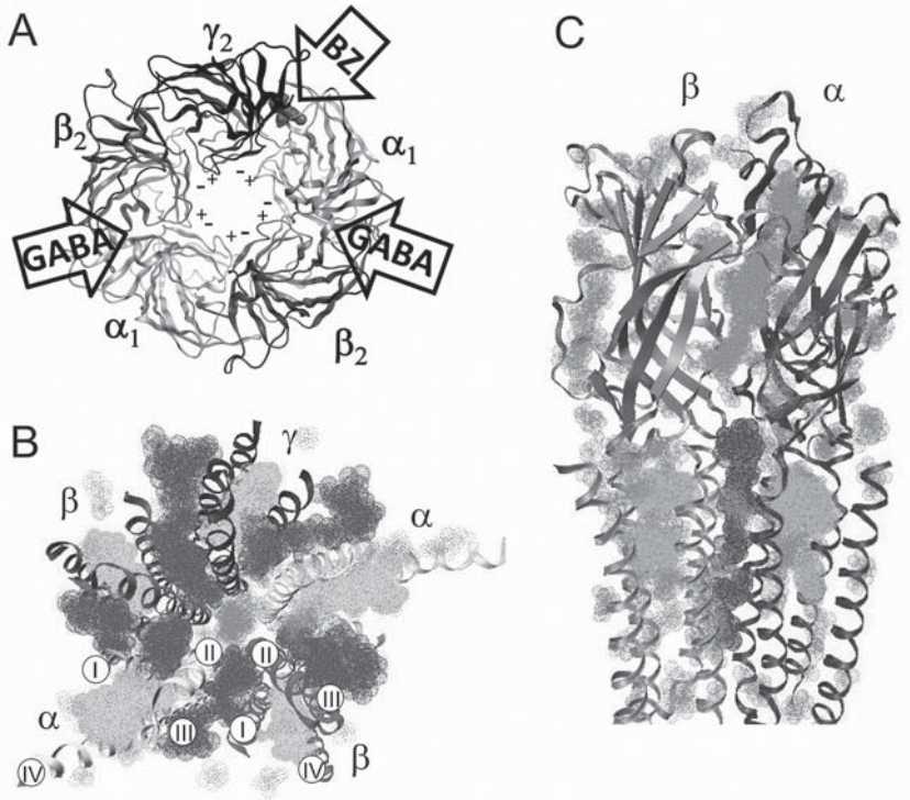
Figure 3: Model structure of the GABA A receptor. (A) Model of the extracellular domain of the GABA A receptor, giving the absolute arrangement for \alpha_1 , \beta_2 , and \gamma_2 containing receptors, the view is from extracellular.
