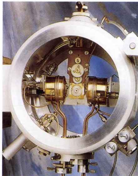
Extreme low-energy ion gun for artifact-free surface layer removal
