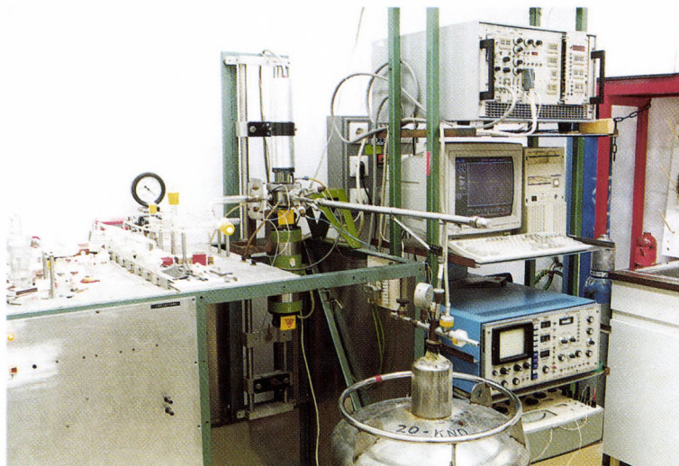
In situ Mössbauer spectrometer Institute of Isotope and Surface Chemistry, Chemical Research Center
