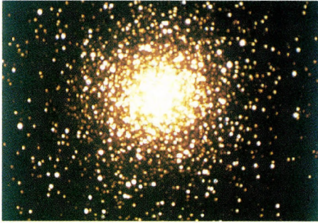
Image of the M3 globular cluster taken with the CCD camera attached on the RCC telescope
