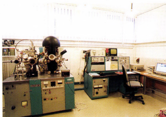
Kratos XSAM-800 type X-ray photoelectron spectroscopic (XPS, ESCA) instrument Research laboratory Materials and Environmental Chemistry, Chemical Research Center
